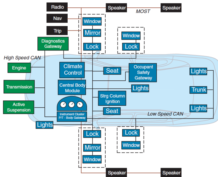
Figure 1-2 Typical Automotive Networks
