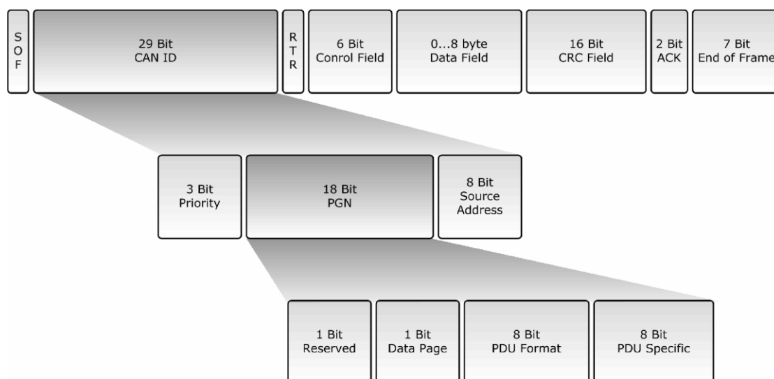
Figure 1-4 J1939 Message Format
