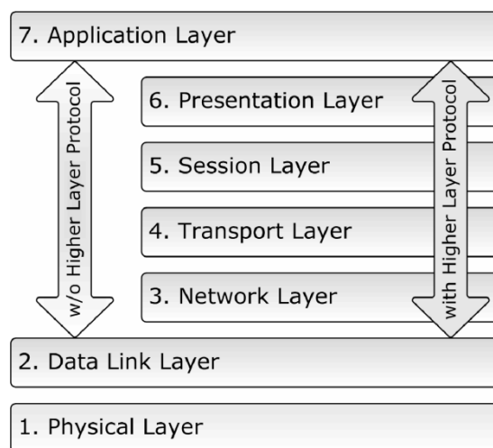
Figure 1-1 ISO/OSI 7-Layer Reference Model
