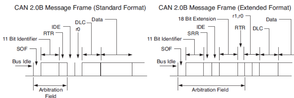
Figure 1-3 CAN Message Formats
